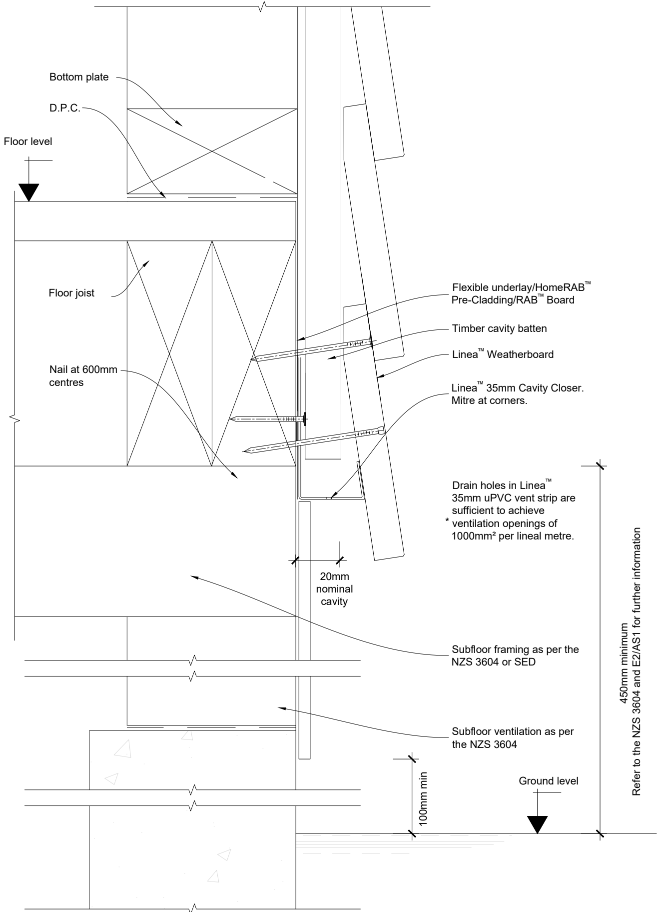
fig40 jhl_junc_c_strc_foun-timb.dwg
